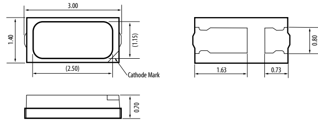
ASMD-LWG3/FWG3 -Nxxxx
