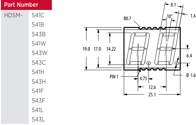
14.22mm (0.56”) Dual Digit SMT Display Package Dimension
