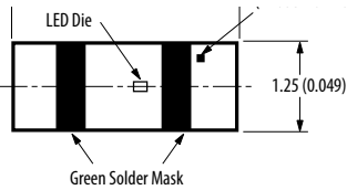
HSMx-C265
