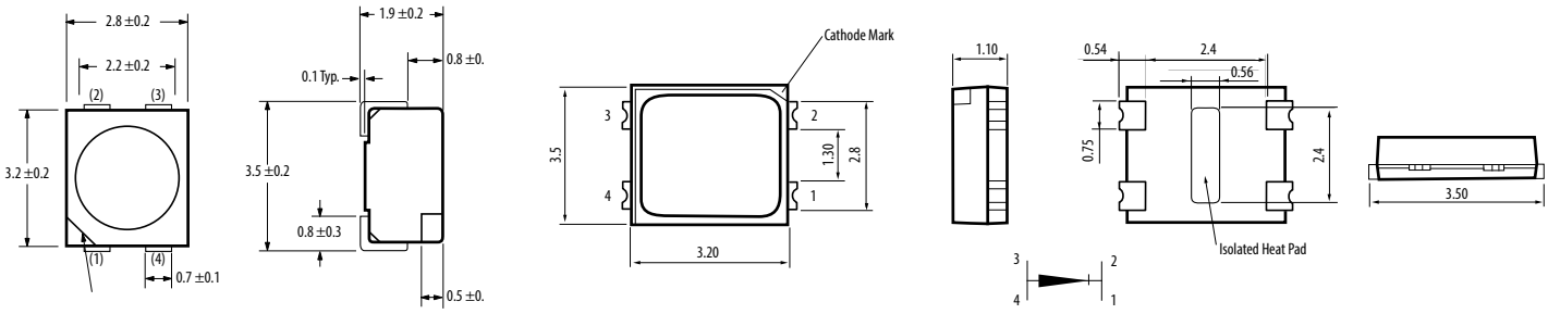
Super 0.5W Power PLCC-4
