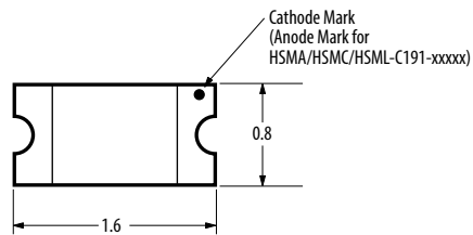
HSMx-C191
