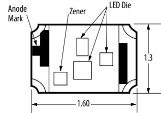
HSMF-C129
