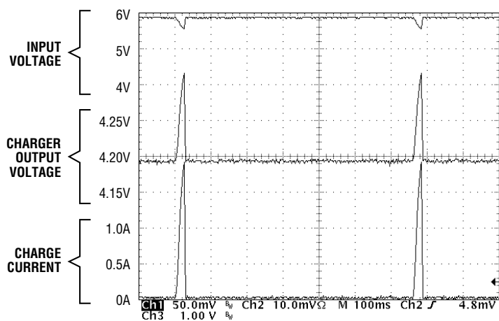
Figure 3. Overcurrent Protection
