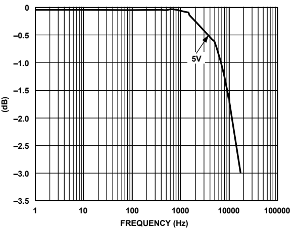
Figure 8. Typical Bandwidth
