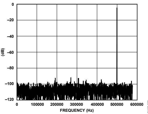
Figure 7. Typical SNR @ 500 kHz Input Tone
