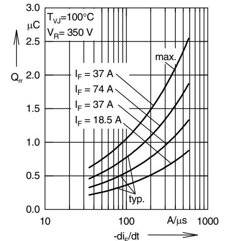
Fig. 11 Recovery charge versus -di_F/dt (Boost Diode)
