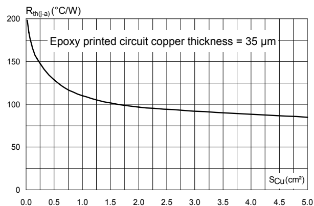
Figure 8. Thermal resistance junction to ambient versus copper surface under each lead (SMA)
