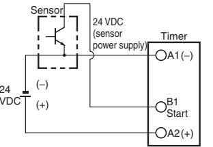
Operates when NPN transistor turns ON.
