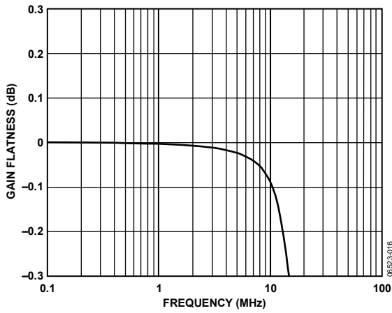
Figure 18. Large-Signal Gain Flatness, V_S = \pm 5\text{ V} , R_L = 150\ \Omega , V_{OUT} = 2\text{ V p-p}
