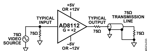
Figure 45. Video Signal Circuit
