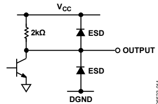
Figure 11. Logic Output
