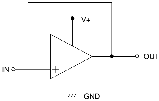
Figure 85. Voltage Follower
