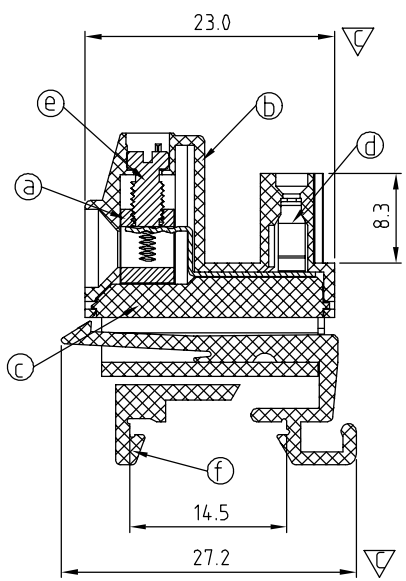
SECTION P-P
