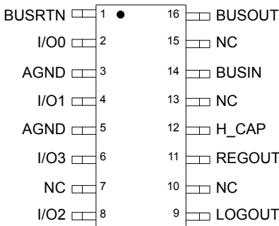
Figure 3. 33793 Pin Connections
