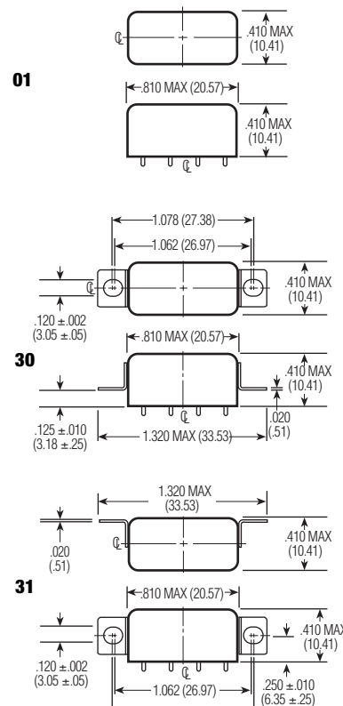
MOUNTING STYLES
