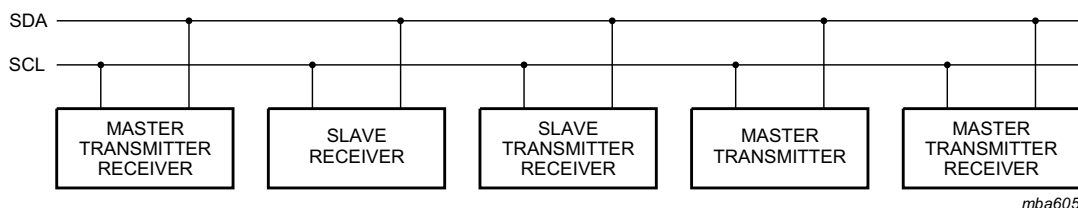
Fig 42. System configuration
