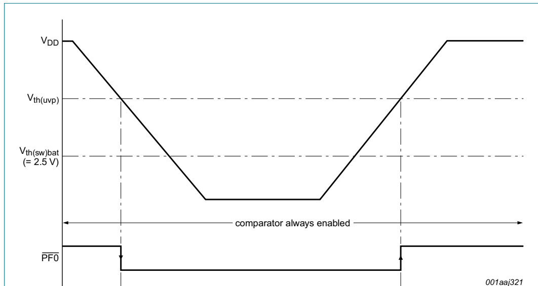
Fig 13. \overline{\text{PFO}} signal behavior when battery switch-over is disabled
