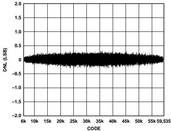
Figure 20. DNL Plot
