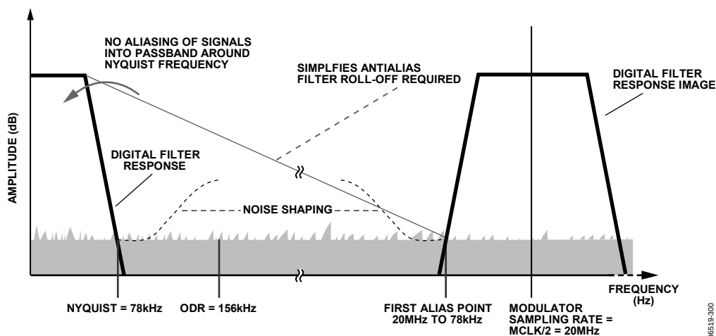
Figure 28. Antialias Example Using the AD7765 in Normal Mode, Decimate 128× Using MCLK/2 = ICLK = 20 MHz
