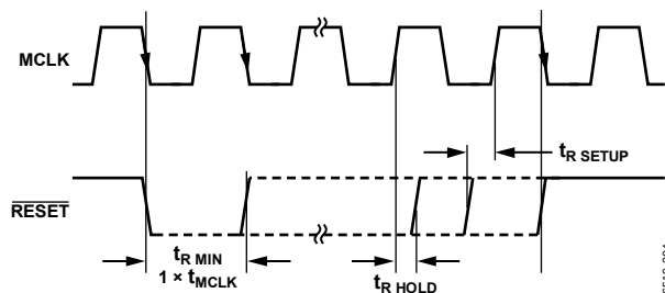
Figure 39. \overline{\text{RESET}} Timing Synchronous to MCLK
