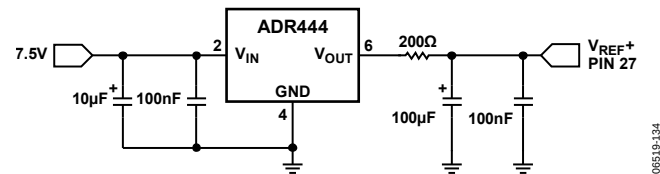
Figure 47. Reference Connection
