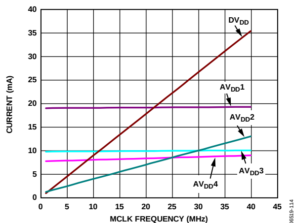
Figure 13. Normal Power Mode; Current Consumption vs. MCLK Frequency, 128x Decimation Rate
