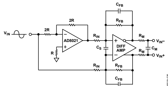
Figure 32. Single-Ended-to-Differential Conversion
