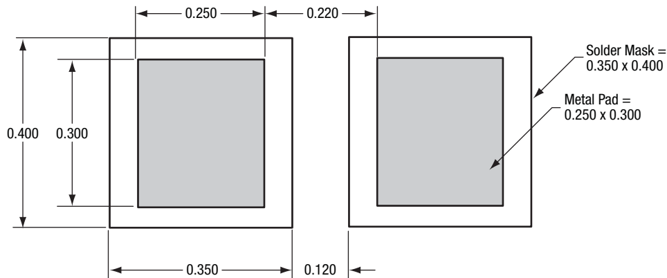
Figure 3. SMS7621-092 PCB Layout Footprint
