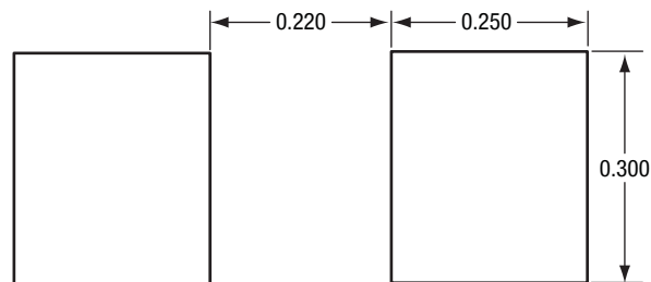
Figure 4. SMS7621-092 Suggested Stencil Aperture
