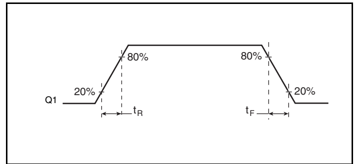
LVCMOS Output Rise/Fall Time
