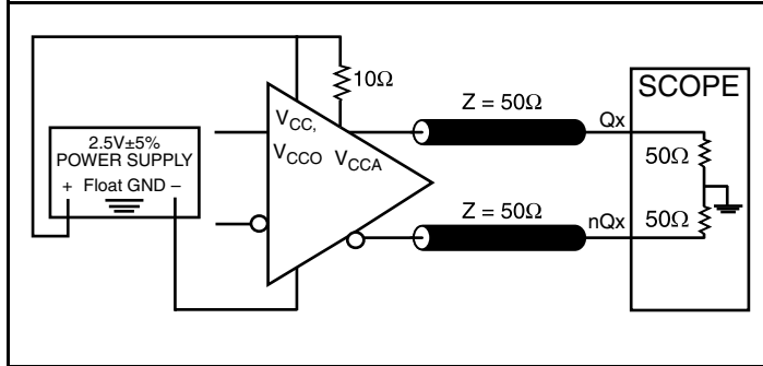
2.5V Core/2.5V LVDS Output Load Test Circuit
