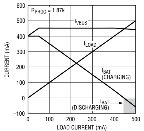
V_{\text{BUS}} and Battery Current vs Load Current
