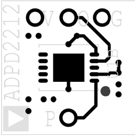
Figure 15. ADPD2212 Evaluation Board Top Layer
