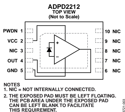
Figure 3. Pin Configuration
