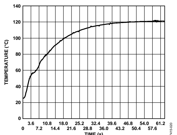
Figure 10. Thermal Step Response in Still Air
