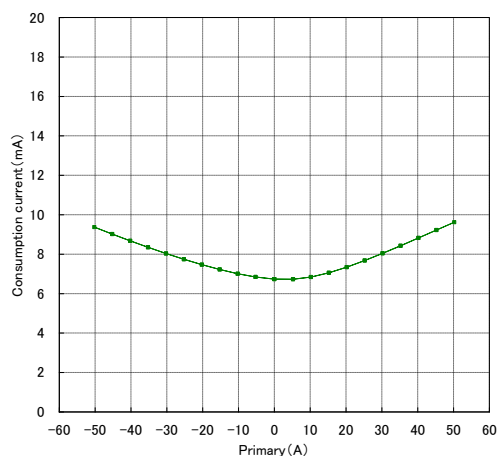
Fig.9-3 Consumption Current
