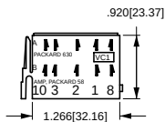
MARKING DETAIL FRONT VIEW VC1 CONNECTOR HOUSING
