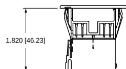
VH1 STANDARD HOLE PLUG (No wing serrations) (With VC1 connector attached)
