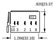
MARKING DETAIL FRONT VIEW VC2 CONNECTOR HOUSING (For AMP terminals only)
