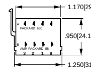
MARKING DETAIL FRONT VIEW VCH CONNECTOR HOUSING
