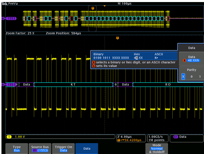
Triggering on a specific data value on the MIL-STD-1553 bus.
