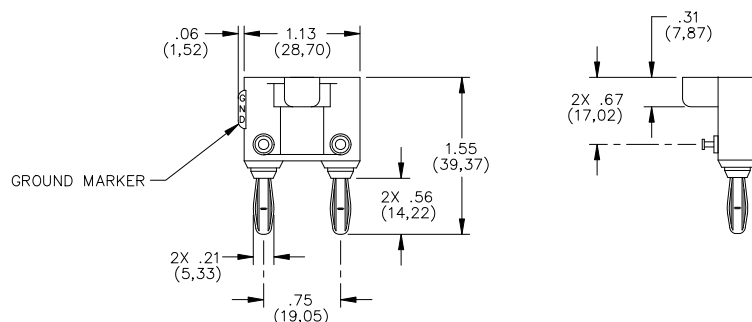
Model MDP-ST Double Banana Plug with Solder Turret Terminals
