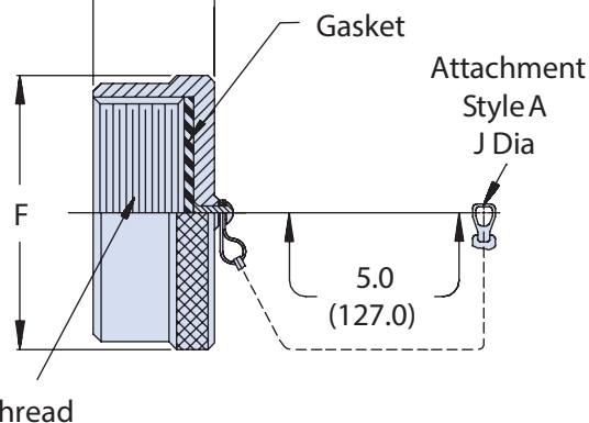
M28840/13 Receptacle Cover
