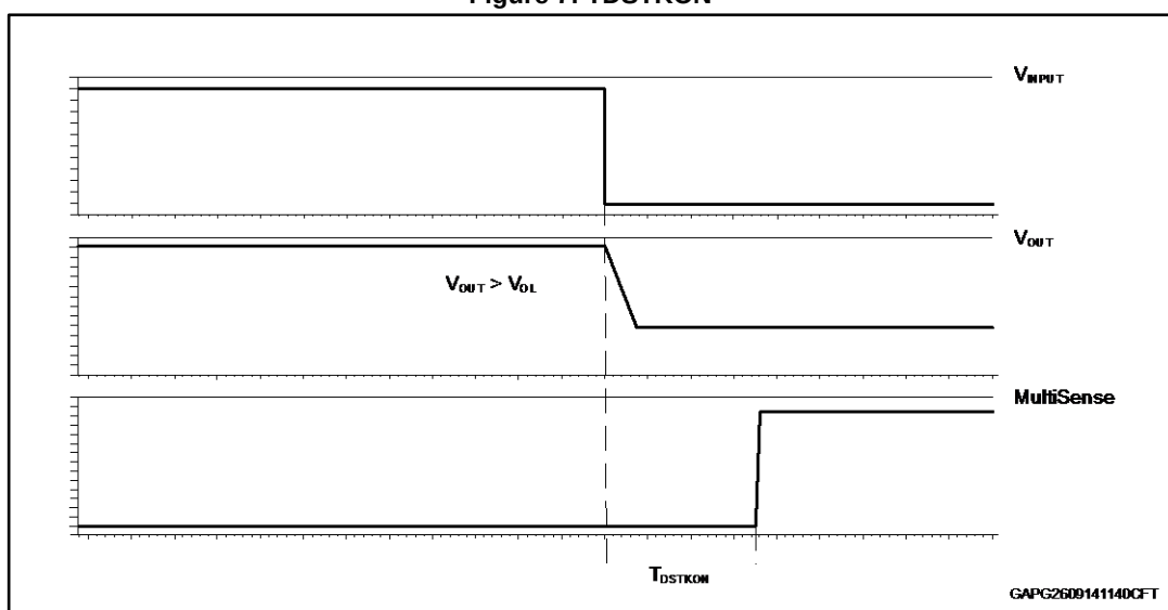
Figure 7: TDSTKON
