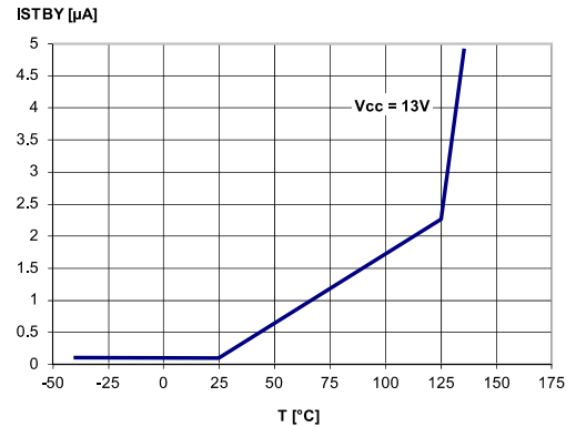
Figure 9: Standby current
