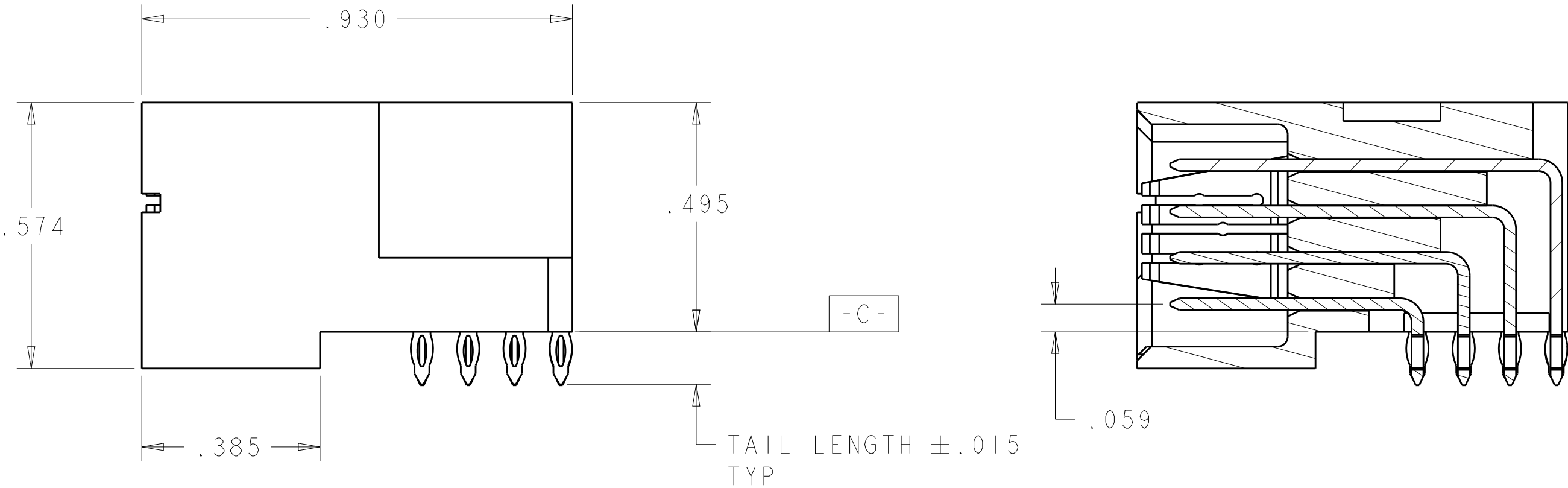
SECTION Z-Z
