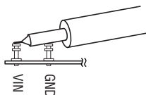
Figure 4. Scope Probe Placement for Measuring Output Ripple
