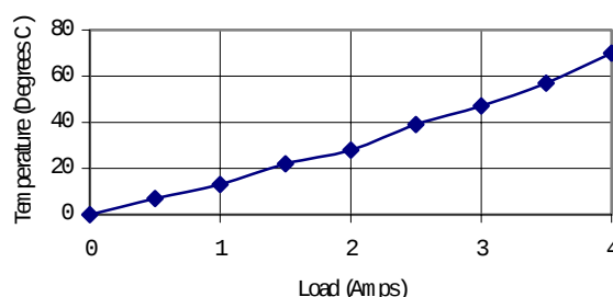
Figure 2. Die Temperature vs Output Current, V_{IN} = 12V
