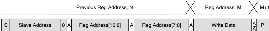
Figure 38. Single WRITE to Random Location
