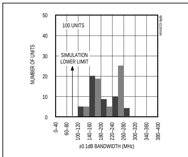
Figure 6b. MAX4224 ±0.1dB Bandwidth Distribution
