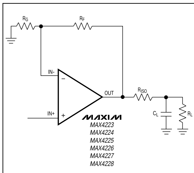
Figure 4. Using an Isolation Resistor ( R_{ISO} ) for High Capacitive Loads
