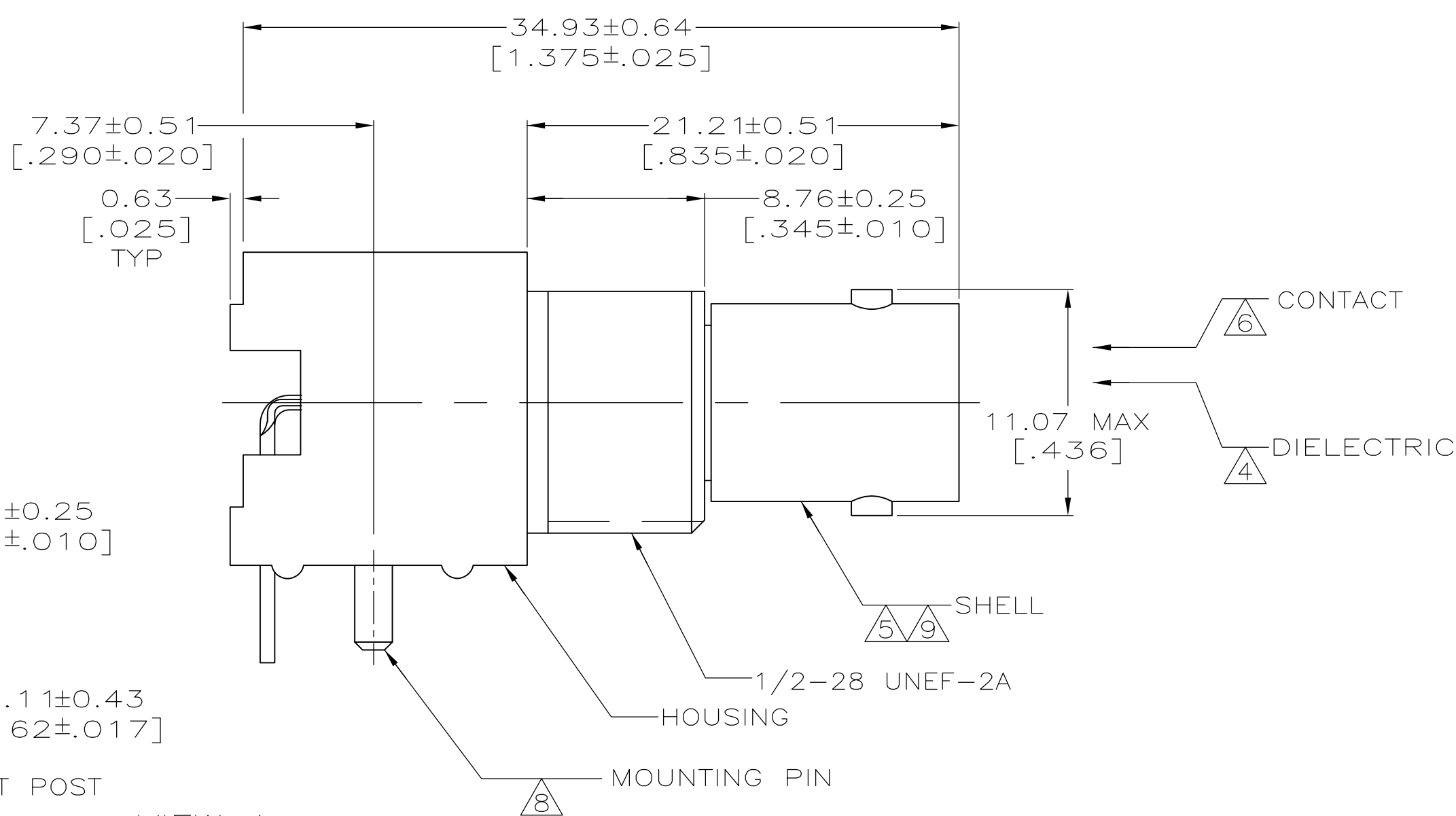
VIEW A
