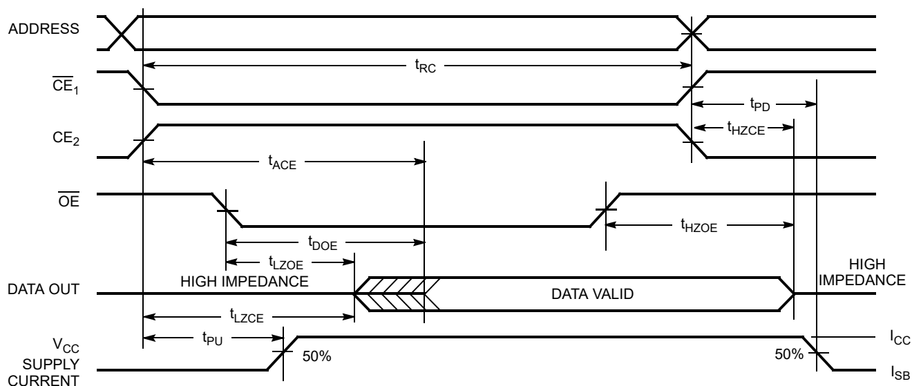
Figure 5. Read Cycle No. 2 ( \overline{OE} Controlled) [23, 24]
