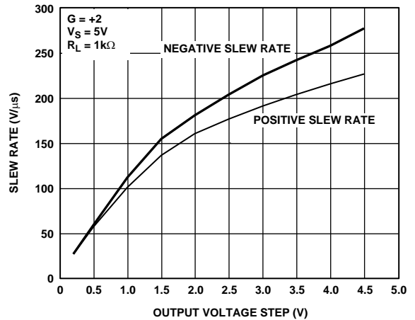
Figure 14. Slew Rate vs. Output Voltage
