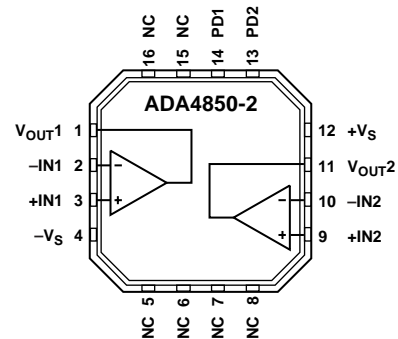
Figure 1. 8-Lead, 3 mm x 3 mm LFCSP
