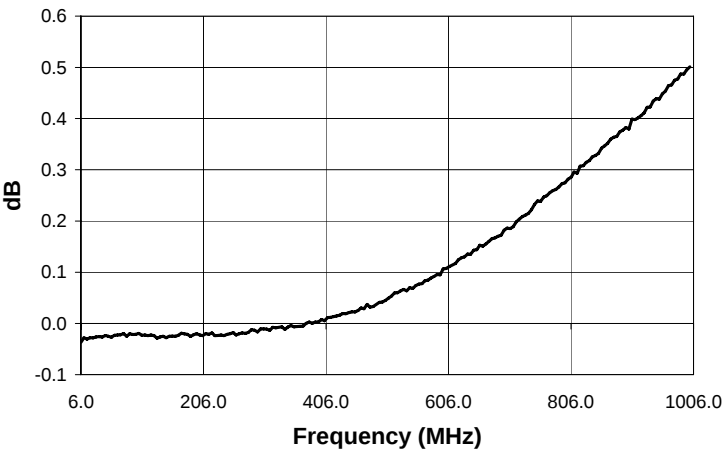
Amplitude Unbalance
