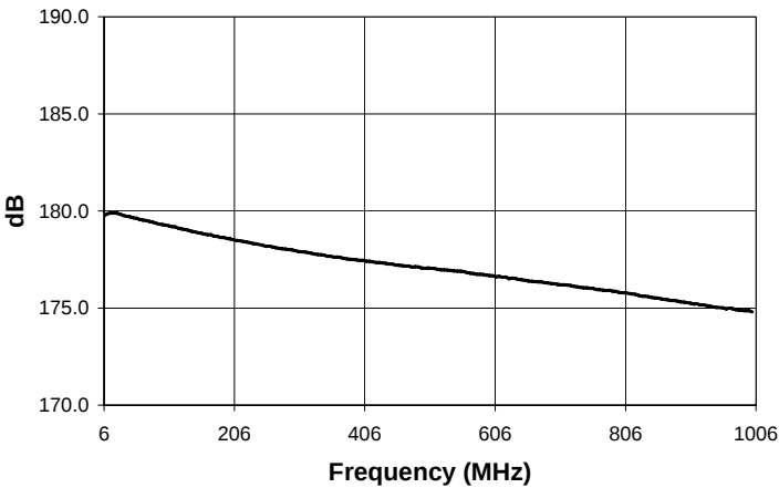
Phase Unbalance
