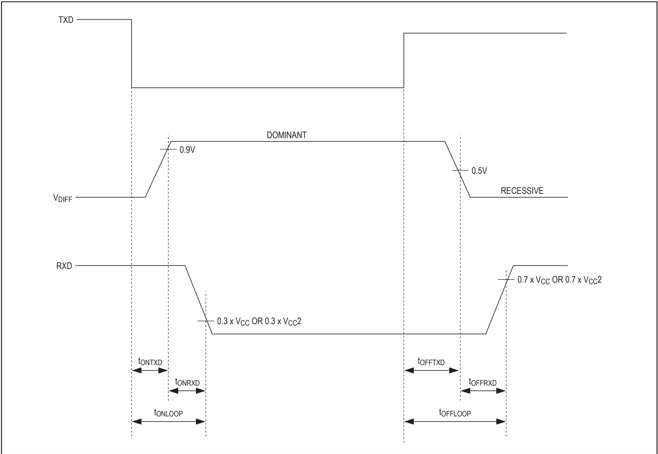
Figure 1. Timing Diagram
