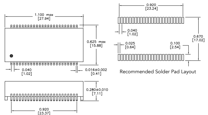
NV6 Package
