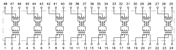
Circuit B
