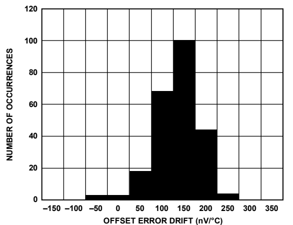
Figure 47. Offset Error Drift, DCLK = 24 \text{ MHz}
