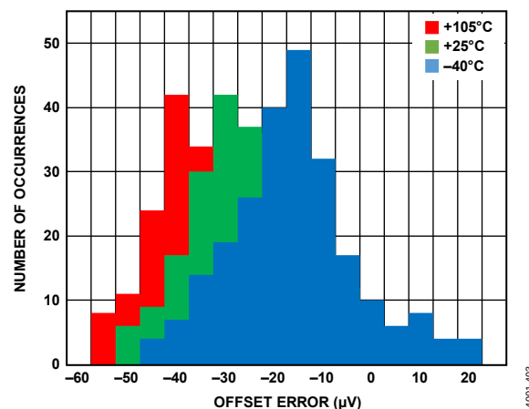
Figure 45. Offset Error Distribution, DCLK = 24 \text{ MHz}
