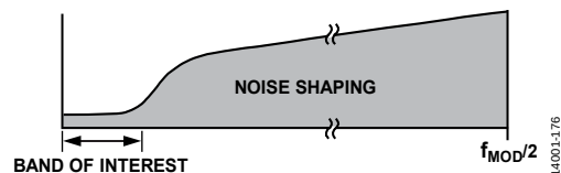
Figure 70. \Sigma - \Delta ADC Noise Shaping (Linear Scale X-Axis)
