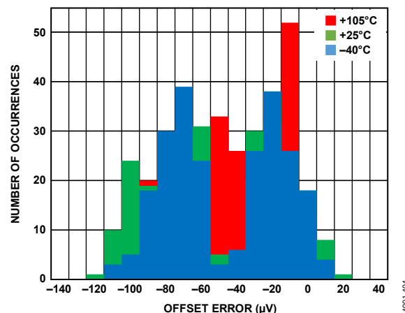
Figure 46. Offset Error Distribution, DCLK = 32 \text{ MHz}
