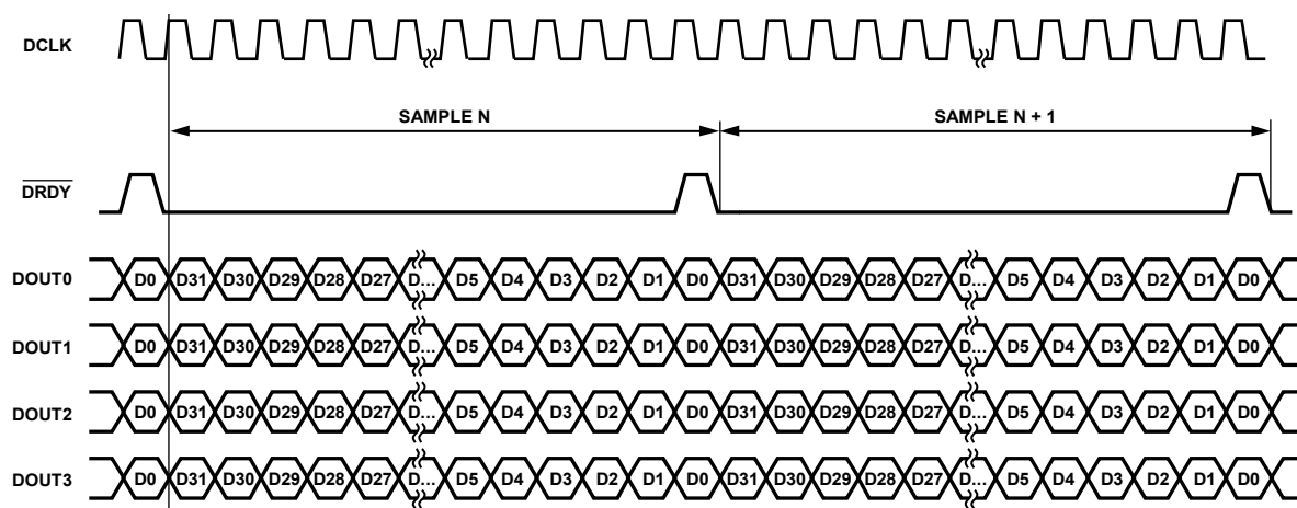
Figure 104. AD7768-4 \text{FORMAT}_0 = 0 : Each ADC Has a Dedicated Data Output Pin, Maximum Data Rate
