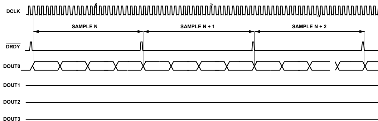
Figure 105. AD7768-4 \text{FORMAT}_0 = 1 : Channel 0 to Channel 3 Output on DOUT0 Only, Maximum Data Rate
