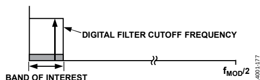
Figure 71. \Sigma - \Delta ADC Digital Filter Cutoff Frequency (Linear Scale X-Axis)
