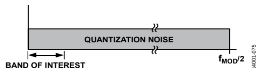
Figure 69. \Sigma - \Delta ADC Quantization Noise (Linear Scale X-Axis)
