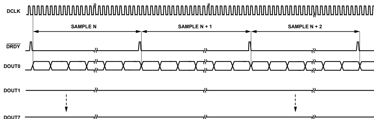
Figure 103. AD7768 \text{FORMAT}_x = 11 or 10 : Channel 0 to Channel 7 Output on DOUT0 Only, Maximum Data Rate
