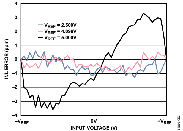
Figure 40. INL Error vs. Input Voltage for Various Voltage Reference ( V_{REF} ) Levels, Fast Mode
