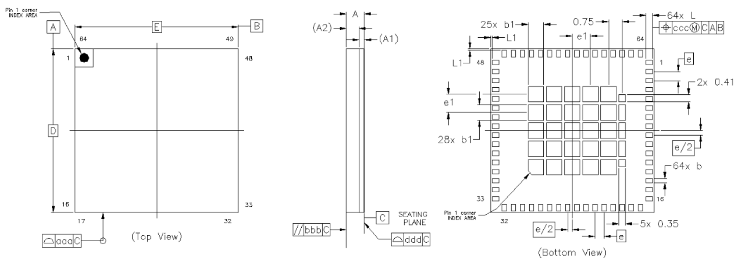
Figure 10.2. 64-Pin LGA
