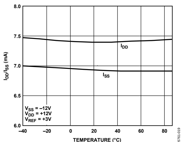
Figure 16. I_{DP}/I_{SS} vs. Temperature
