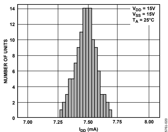
Figure 17. Typical I_{DP} Distribution
