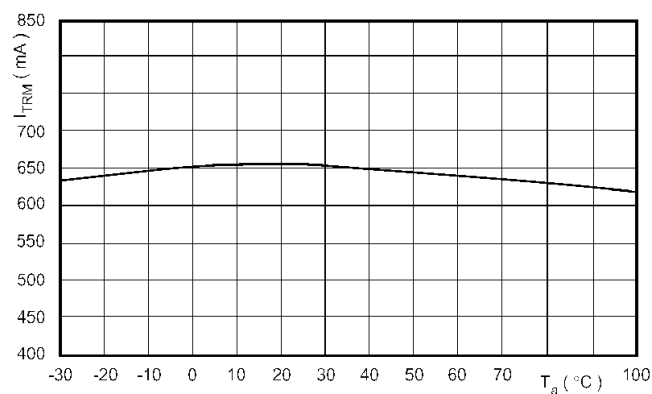
Trigger current at 10 V vs. temperature, V_{CC} = 10 V
