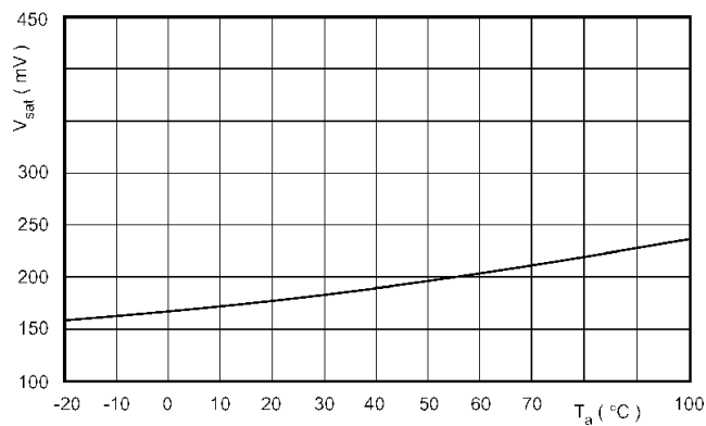
Timer output saturation voltage at 1mA V_{CC} = 10 V
