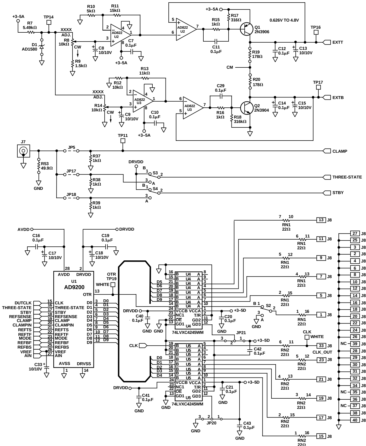
Figure 39a. Evaluation Board Schematic
