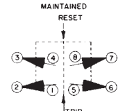
DPDT Double Break (Electrical rating B)
