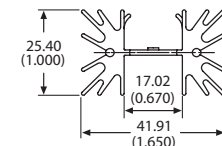
VIEW A-A SINGLE HEAT SINK DEVICE
