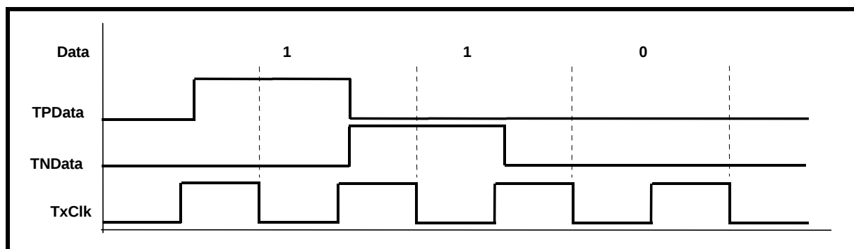
FIGURE 15. THE XRT73LC04A SAMPLES THE DATA ON THE TPDATA AND TNDA INPUT PINS
