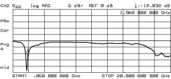
S11, S22 (~20GHz)
