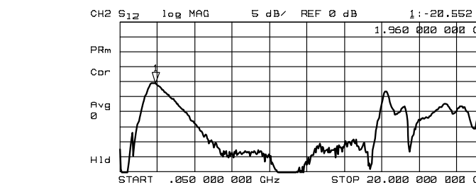
S21, S12 (~20GHz)
