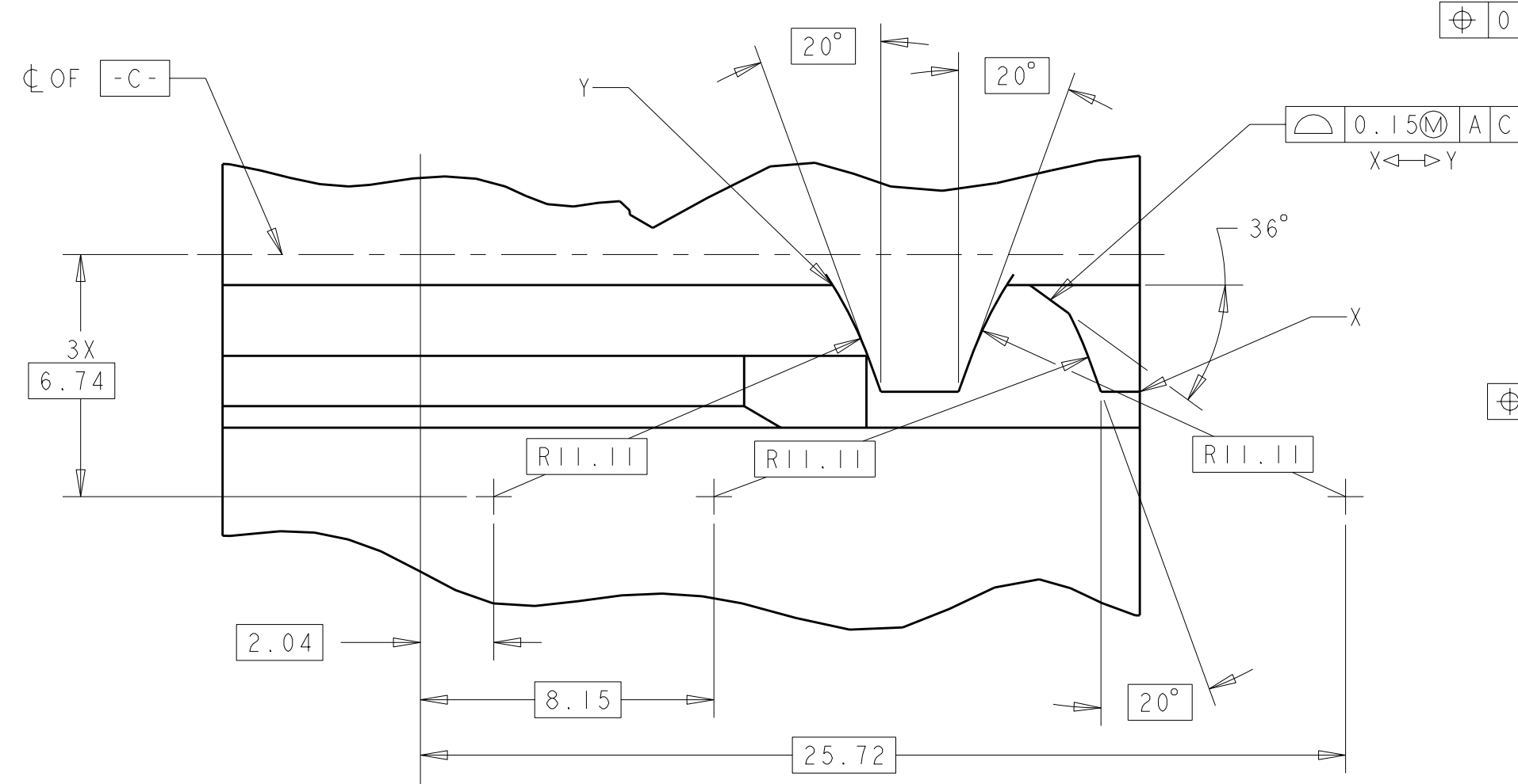
DETAIL G SCALE 6:1 2 PLC
