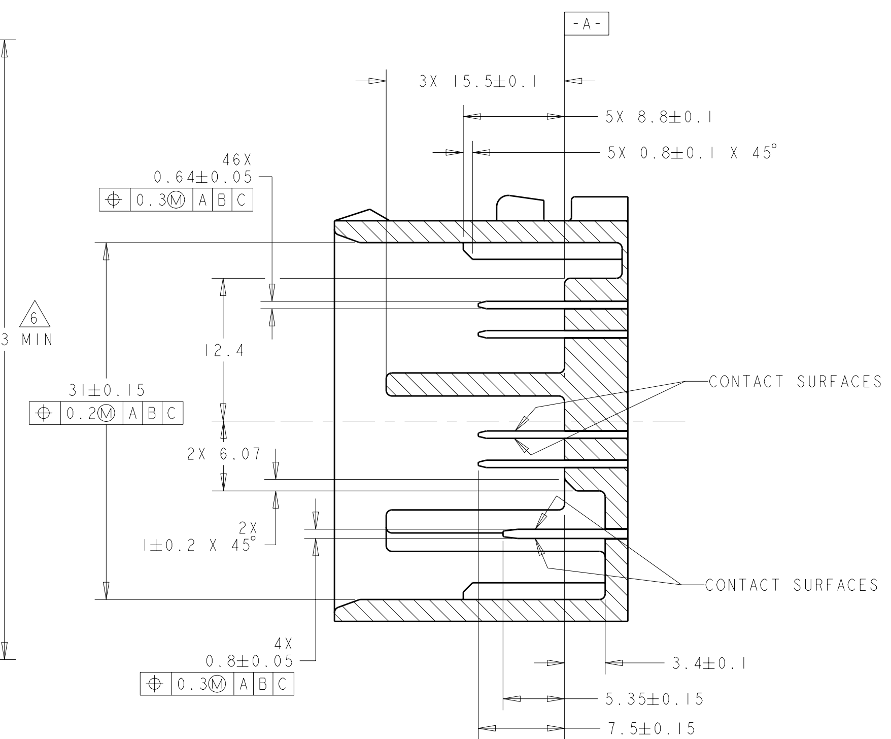
SECTION B-B
