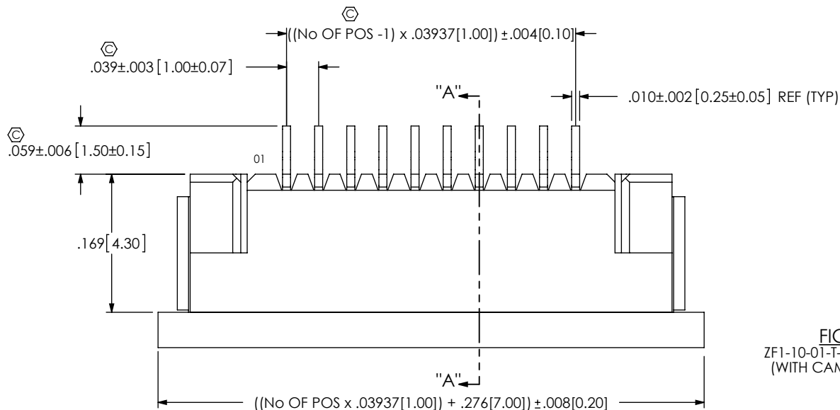
BACK VIEW
